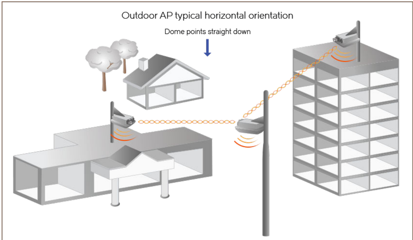
FIGURE 305 Outdoor AP typical horizontal orientation
